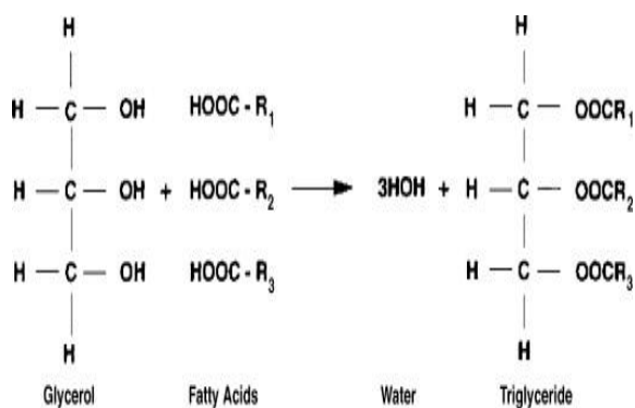
Fig 1: Chemical Structure of Vegetable Oils
