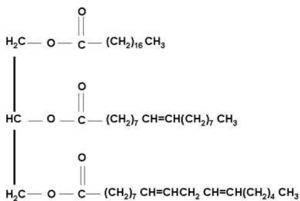
Fig 2: Structure of a Typical Triglyceride Molecule
