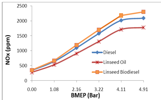
Fig 6: Variation of Oxides of Nitrogen with Brake Mean Effective Pressure
