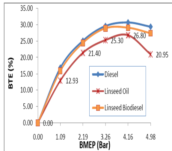
Fig 4: Variation of Brake Thermal Efficiency with Brake Mean Effective Pressure
